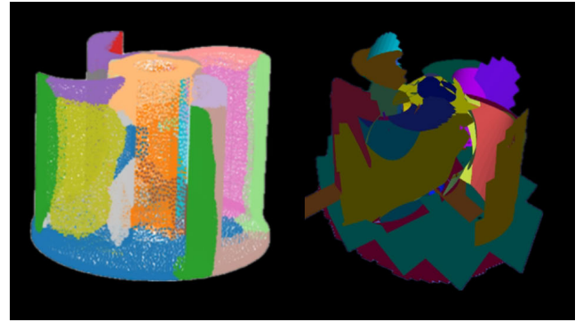
FIGURE 6. An example of cross-boundary layer misassignment for a component with increased complexity. The error is localized to ambiguous high-curvature junctions where the upstream segmentation merges adjacent surfaces (Sec. VIII-E); it does not reflect a failure of the contact-aware solver.
