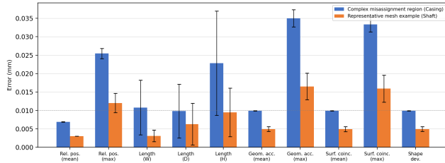
FIGURE 9. Case-wise mean relative errors (in mm) under the current artifact protocol for the complex misassignment region and a representative mesh example.
