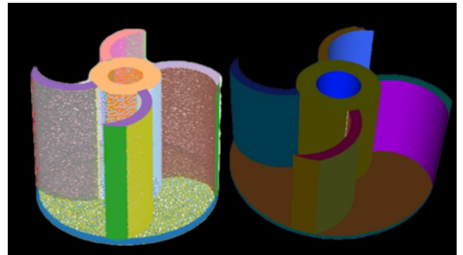
FIGURE 7. Successful reconstruction of the same casing component shown in Fig. 6: a watertight mesh/B-rep with preserved free-form surfaces and valid topology, obtained on a run in which the upstream segmentation separated the ambiguous junction correctly. This confirms that the misassignment in Fig. 6 is a run- and scan-dependent segmentation artifact, not a systematic failure of the contact-aware solver.
